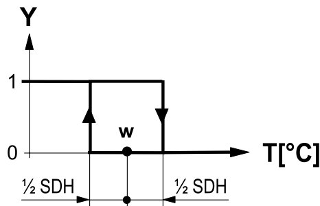
Control sequence
